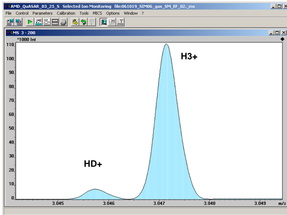
Fig. 1 high resolution isotope separation HD+ and H3+ ion doublet
