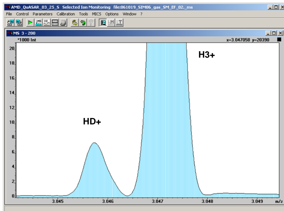
Fig. 2 high resolution isotope separation HD+ and H3+ ion doublet at extended scale
