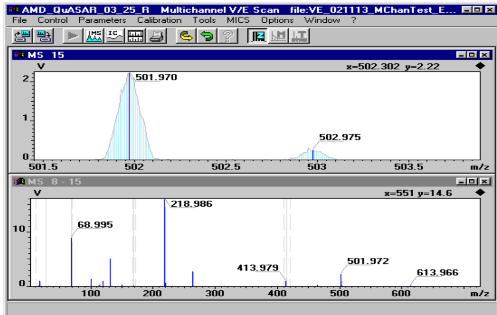
Fig. 3 Rapid electric V/E scans over full mass range with Multi Channel Detection (EI)
