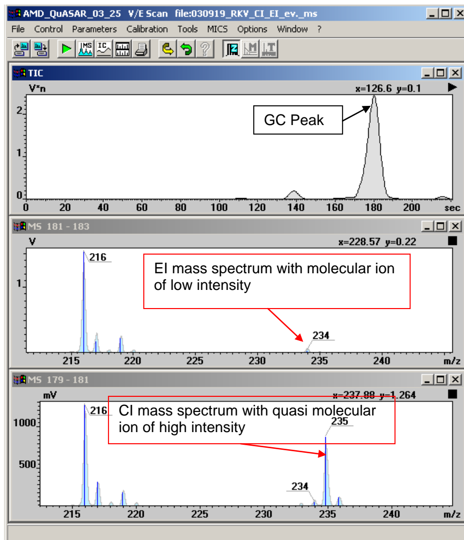
Fig. 5 GC/MS V/E scans using unique EI/CI-UDIC arrangement for alternating Spectra in EI and CI mode within one GC peak
