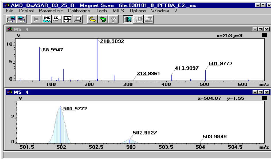
Fig. 1 Magnet Scan at medium resolution (EI)
