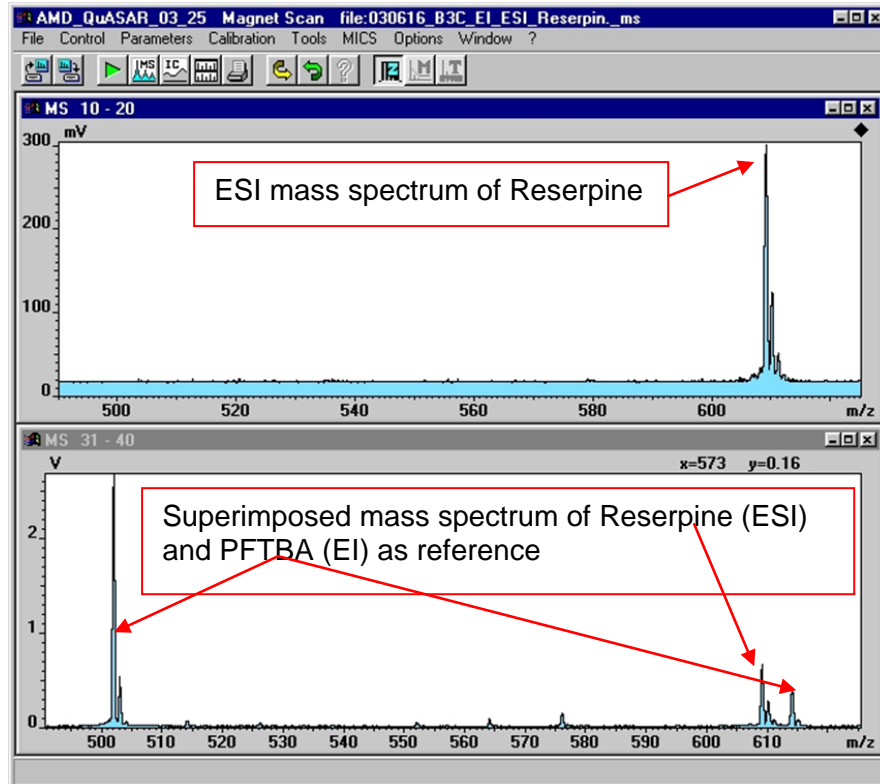
Fig. 4 Magnet scans with simultaneous recording of EI and ESI ions using unique API interface
